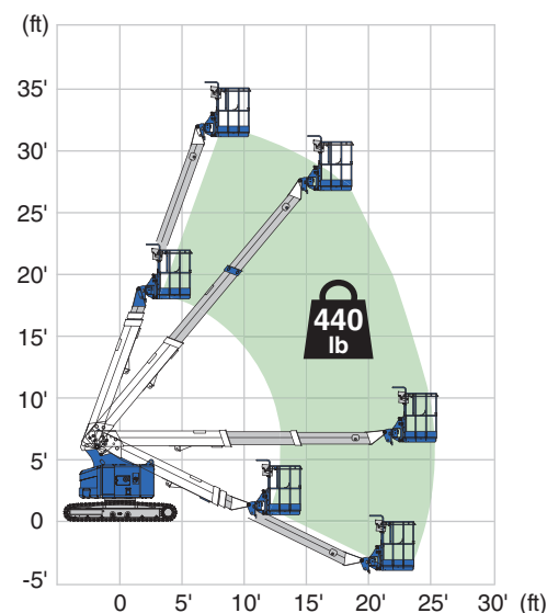
AS-32C Range of motion
