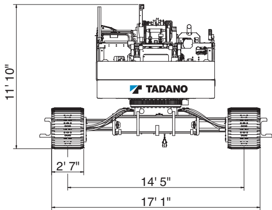
Tracks extended
