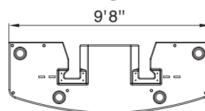
Counterweight „B“ section
